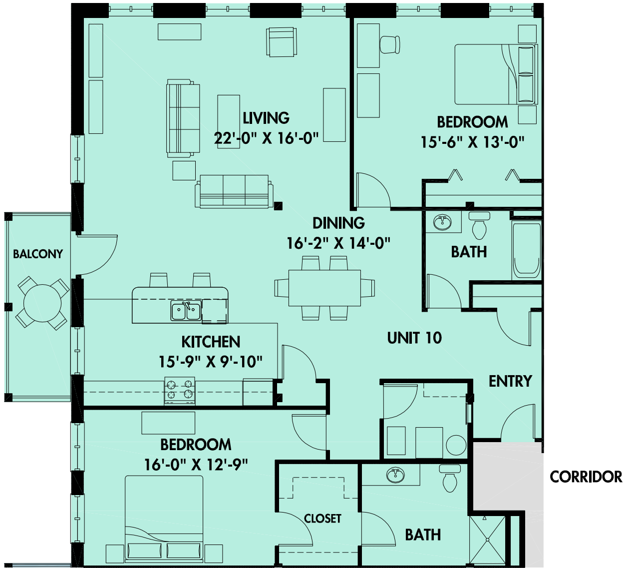
Two Bedroom 1720 Square Feet Dimensions and Area are approximate
